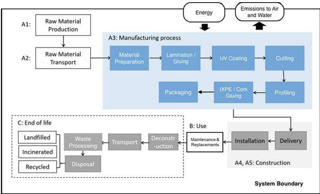
Figure 3. System Boundary
